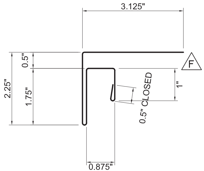
PF55 F AND J TRIM ( \frac{1}{2} " TO \frac{3}{4} ")
